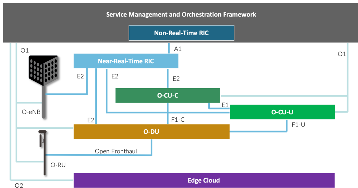
Figure 6: O-RAN Architecture
