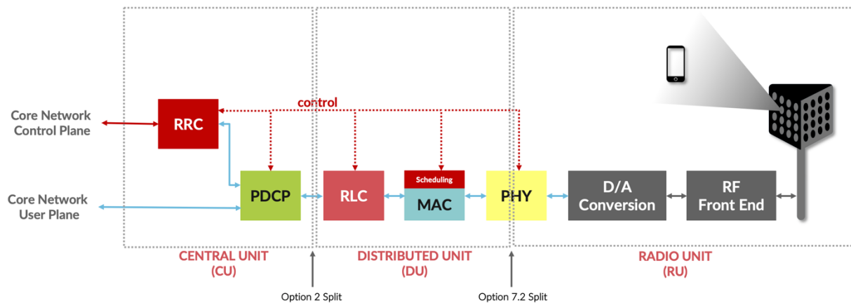
Figure 4: CU-DU-RU Disaggregation
