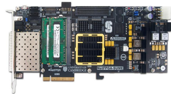
NetFPGA SUME 4x10G ports
